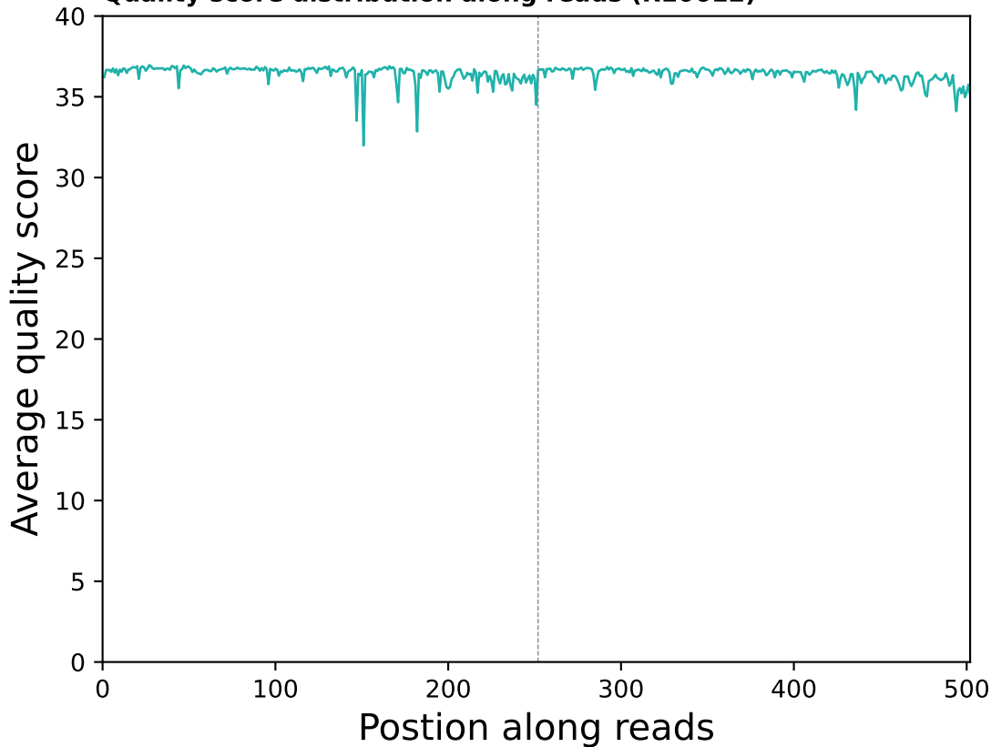
Quality score distribution along reads (R10612)
